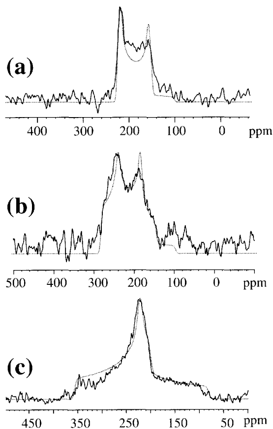
Fig. 2. Experimental (solid lines) and calculated (broken lines) ^{67}\text{Zn} MAS spectra of (a) natural abundance \text{Zn}(\text{CH}_3\text{COO})_2 (number of scans, 32 225; spinning rate, 8.5 kHz; recycle delay, 1 s), (b) ^{67}\text{Zn} -enriched \text{Zn}(\text{imidazole})_4(\text{ClO}_4)_2 (number of scans, 16 774; recycle time, 1 s; spinning rate, 8.1 kHz), and (c) ^{67}\text{Zn} -enriched \text{Zn}(\text{thiourea})_4(\text{NO}_3)_2 (number of scans, 19 188, recycle time, 2 s; spinning rate, 9.1 kHz).
