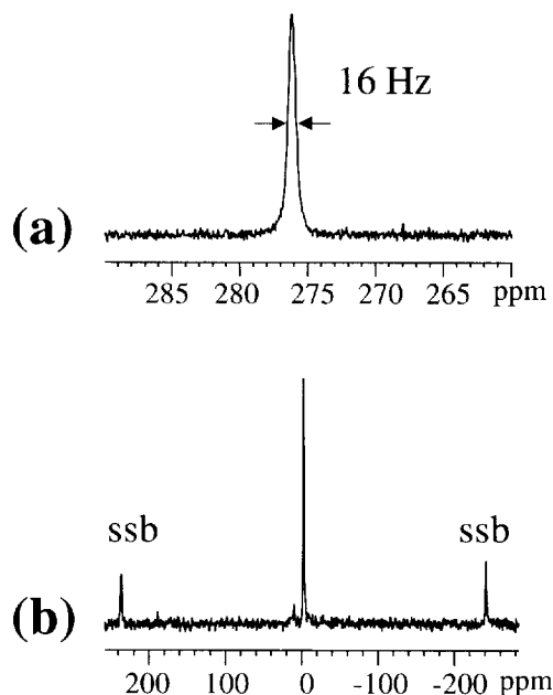
Fig. 1. ^{67}\text{Zn} MAS spectra of (a) natural abundance \text{ZnSe} (number of scans, 360; recycle delay, 1 s; spinning rate, 5.0 kHz) and (b) ^{67}\text{Zn} -enriched \text{Zn}(\text{ClO}_4)_2 \cdot 6\text{H}_2\text{O} (number of scans, 128; recycle delay, 10 s; spinning rate, 6.0 kHz). Spinning sidebands are marked as "ssb."
