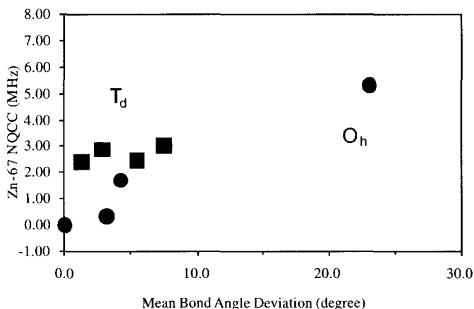
Fig. 4. Plot of ^{67}\text{Zn} NQCC versus mean bond angle deviation from perfect T_d (■) and O_h (●) symmetry.
