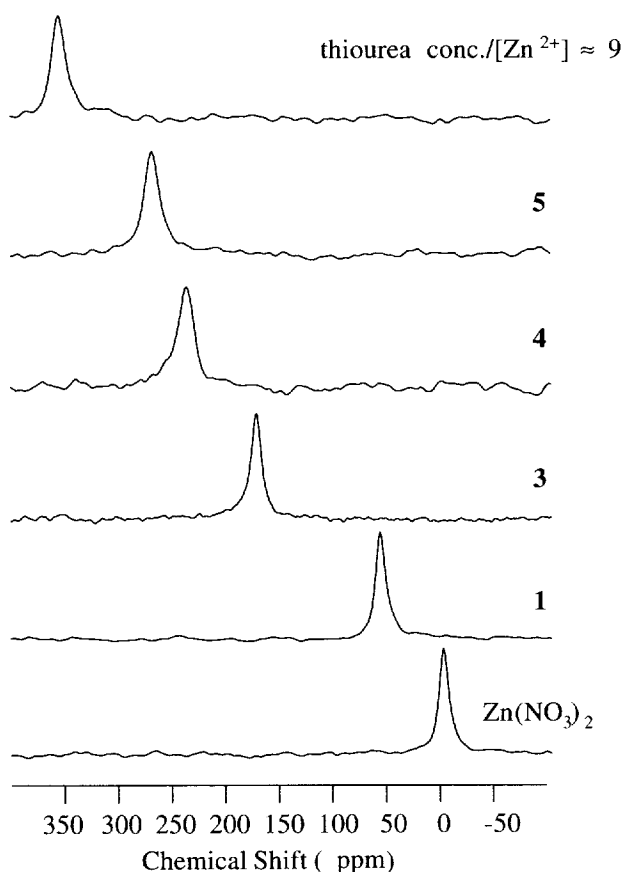
Fig. 3. ^{67}\text{Zn} NMR spectra of aqueous solutions of \text{Zn}(\text{NO}_3)_2 and thiourea at different thiourea conc./ [\text{Zn}^{2+}] ratios. The pH value of the solution varies from 4.20 (1:1) to 3.78 (1:9).
